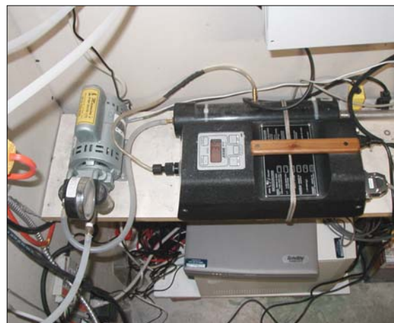
Figure 5 – Rotronic Temperature/Humidity Transmitter (incoming sewer air)
